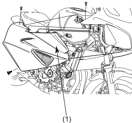
(1) Panel lateral
